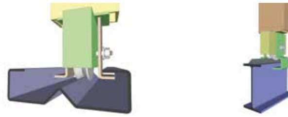
Ground-side and overhead running wheels
